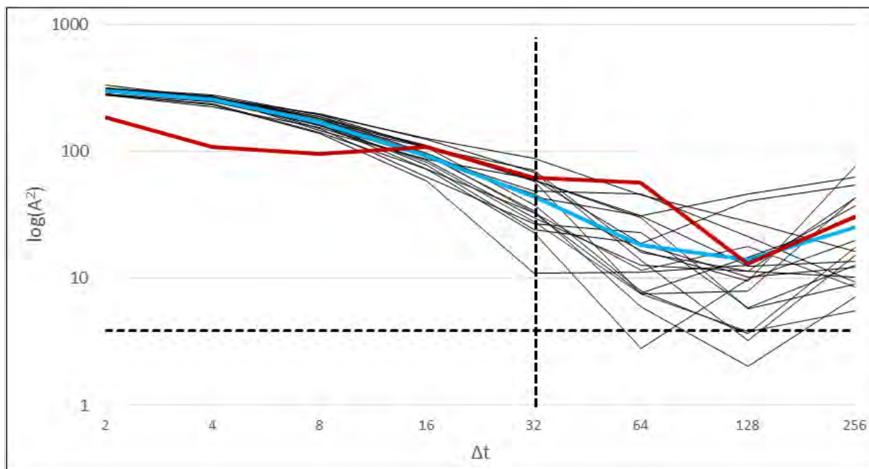
Figure 23. Log-scaled Anderson-Darling test statistic values for the 20 replications of 1,000 artificial data points each using the Cauchy(0,1) as \varphi and n = 2 for different delay values \Delta . The critical value for all replications 3.907.
